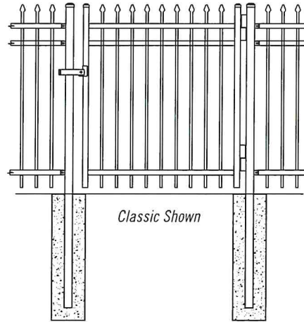
SINGLE SWING DIMENSIONAL DRAWING
