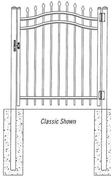
SINGLE SWING DIMENSIONAL DRAWING
