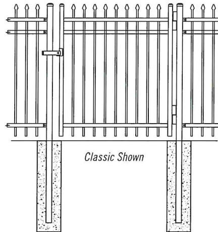
HGBS-25 HGBS-3 / HGBS-4 HEAVY COMMERCIAL HINGE KITS IGBS-25 IGBS-3 / IGBS-4 INDUSTRIAL HINGE KITS
