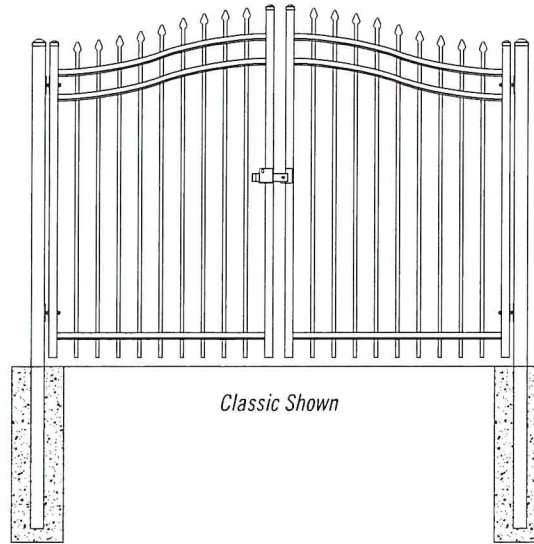
DOUBLE SWING DIMENSIONAL DRAWING
